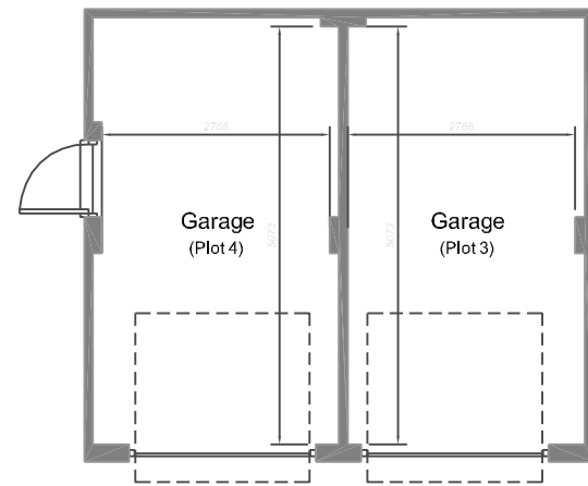
Garage Plan
